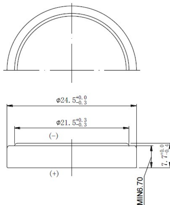
Dimension Drawing
