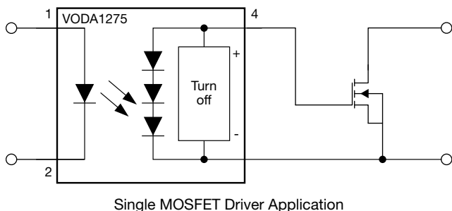
Single MOSFET Driver Application
