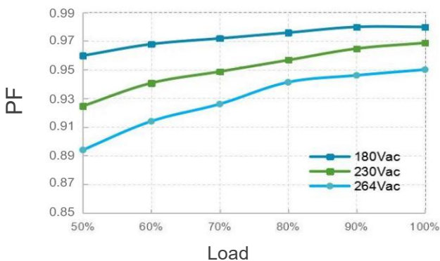
Power Factor (PF) Curves
