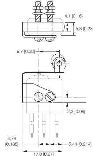
Figure 13. JM-5 Dimensions
