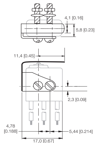
Figure 12. JM-1 Dimensions
