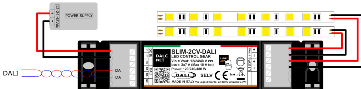
Figure 3: Wiring diagram for White or Single-Colour LED loads
