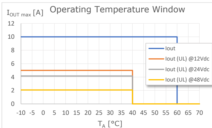
Figure 10: Operating Temperature Window
