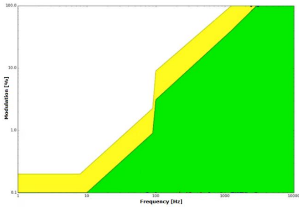
Figure 9: Flickering Perception Threshold
