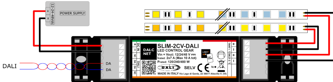
Figure 4: Wiring diagram for Dim-to-Warm & Tunable-White dimming on separate loads
