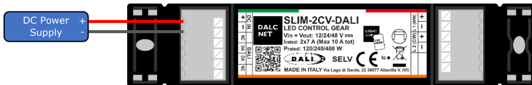
Figure 8: Power Supply wiring Diagram
