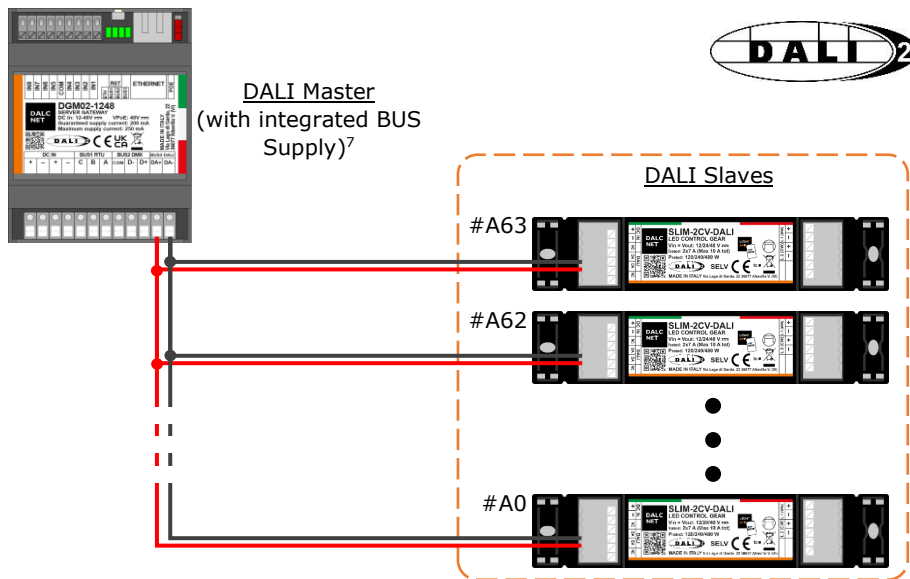
Figure 7: Remote Control Connection Topology, Bus-wiring
