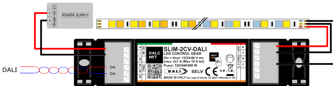
Figure 5: Wiring diagram for Dim-to-Warm and Tunable-White dimming on a single load
