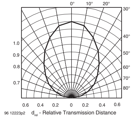
Fig. 12 - Horizontal Directivity
